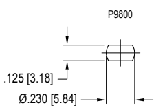
SCREW COLLAR CUTOUTS PRESS FIT
